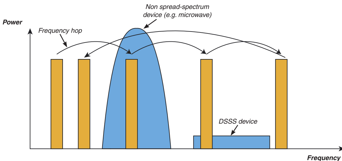
Figure 4: FHSS probe transmission co-existing with other radio traffic
