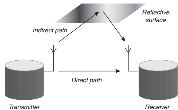
Figure 5: radio waves reflect off surfaces inside the machine tool and can interfere with waves travelling on a direct path to the receiver. Frequency hopping avoids 'dead spots' by regularly switching channels
